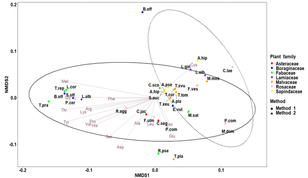
Fig 2. nMDS ordination plot based on Bray-Curtis distances calculated on amino acids contents (i.e., amounts in µg/mg of amino acids) from pure floral pollen for each plant species (stress = 0.09). Method 1: IEX chromatography method; Method 2: HPLC method. The two ellipses gather species according to the analytical method used with solid lines for the IEX chromatography method and dashed lines for the HPLC method. Families are indicated in different colours. Amino acids: Ala, alanine; arg, arginine; asp, aspartic acid; cys, cysteine; glu, glutamine; gly, glycine; his, histidine; ile, isoleucine; leu, leucine; lys, lysine; met, methionine; phe, phenylalanine; pro, proline; ser, serine; thr, threonine; tyr, tyrosine; val, valine. Species: A.pla, Acer platanoides ; A.pse, Acer pseudoplatanus ; A.car, Aesculus carnea ; A.hip, Aesculus hippocastanum ; B.off, Borago officinalis ; C.jac, Centaurea jacea ; C.lae, Crataegus laevigata ; C.seg, Cyanus segetum ; C.sco, Cytisus scoparius ; E.vul, Echium vulgare ; F.ulm, Filipendula ulmaria ; F.ves, Fragaria vesca ; L.alb, Lamium album ; L.gal, Lamium galeobdolon ; L.cor, Lotus corniculatus ; M.mos, Malva moschata ; M.dom, Malus domestica ; P.avi, Prunus avium ; P.cer, Prunus cerasus ; P.com, Pyrus communis ; R.pse, Robinia pseudoacacia ; R.agg, Rubus aggr. ; S.auc, Sorbus aucuparia ; S.off, Symphytum officinale ; T.cor, Tilia cordata ; T.pra, Tilia platyphyllos ; T.tom, Tilia tomentosa ; T.xeu, Tilia x euchlora ; T.xvu, Tilia x vulgaris ; T.pra, Trifolium pratense ; T.rep, Trifolium repens .
