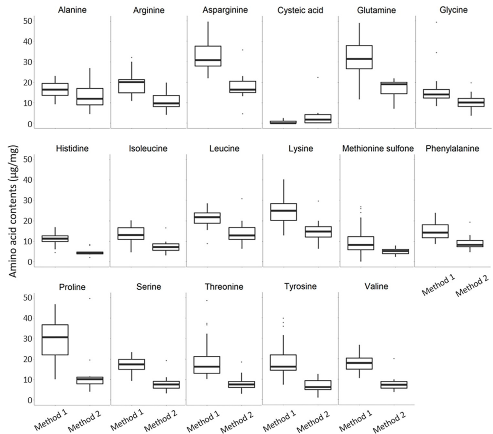
Fig 3. Boxplots of the contents of each amino acid ( \mu\text{g}/\text{mg} ) according to the IEX chromatography method (Method 1) and the HPLC method (Method 2).
