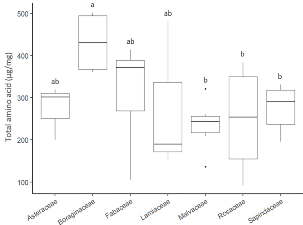
Fig 1. Boxplot of total amino acids per plant family.
