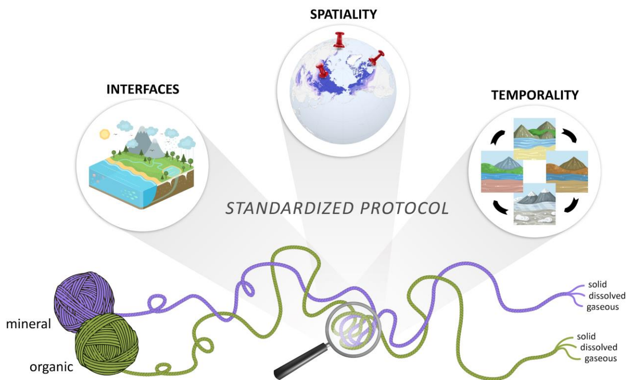
Figure 1 The mineral and organic permafrost pools.
